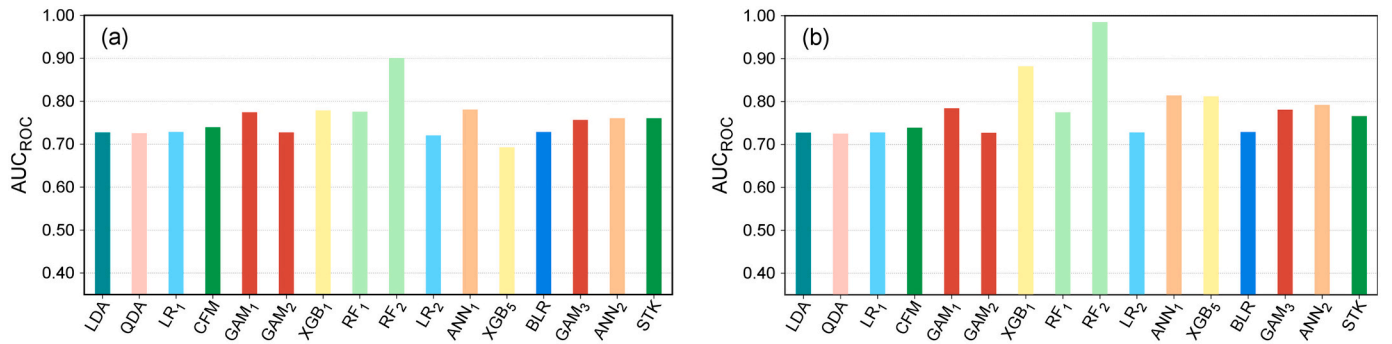
Fig. 14. Comparison of AUC_{ROC} values for the different methods considered in step two of the experiment (Section 5), limited to the p_1 landslide flag. Values in (a) were calculated by the contributors, and values in (b) were obtained by the organizers of the experiment calculating AUC_{ROC} from the attribute tables provided by the contributors. Names of the different methods are as in Fig. 3, Sections 4.1–4.11.
