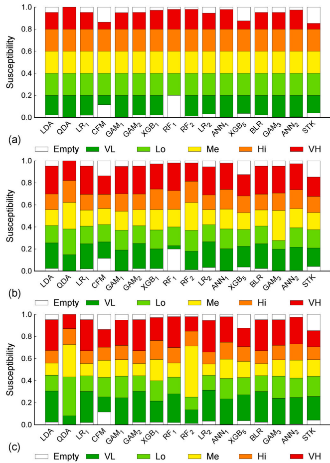
Fig. 20. Stacked bars representing different class breaks, for the p1 scenario, using (a) equal intervals (same breaks, different number of values in each class; used in Fig. 17), (b) Jenks natural breaks (different breaks and different number of values in each class), and (c) percentiles of the distributions (different breaks, but each class contains the same number of values, i.e., of slope units). In all cases, we show the actual lower and upper limits in the distribution of susceptibility values with a white band.
